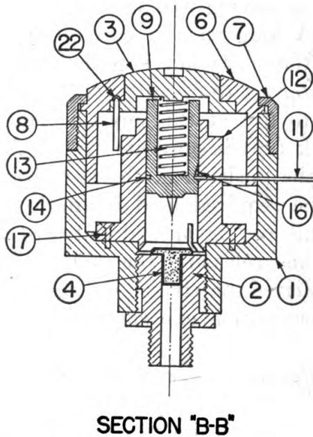
FIGURE 10.—Combined igniter Z. D. Z. 29.
